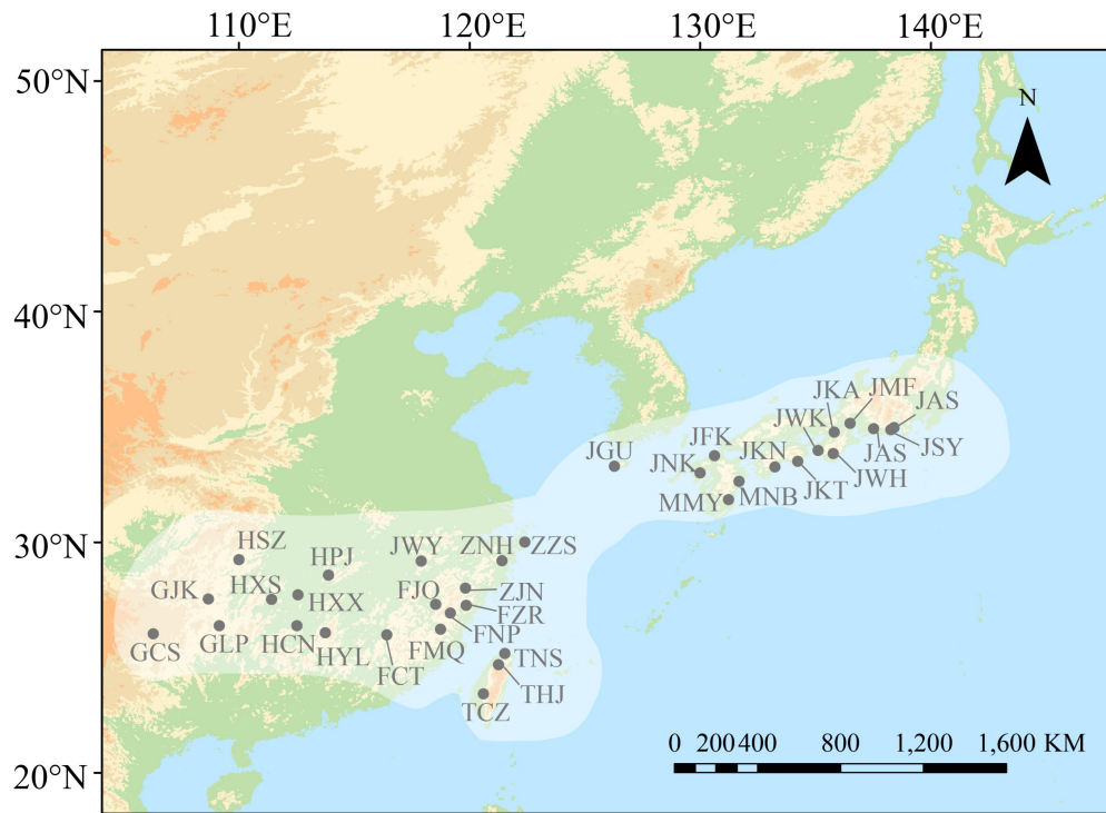
Supplementary Fig. S1 The geographical distribution of Quercus gilva . Black dots on the map represent our field collection sites.
