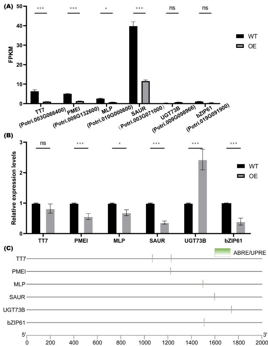
Figure S6 Expression pattern of potential targets of PagbZIP60 verified by RT-qPCR. (A-B) Expression pattern analyzed using RNA-seq and RT-qPCR. (C) The ABRE/UPRE cis -acting elements in promoters.
