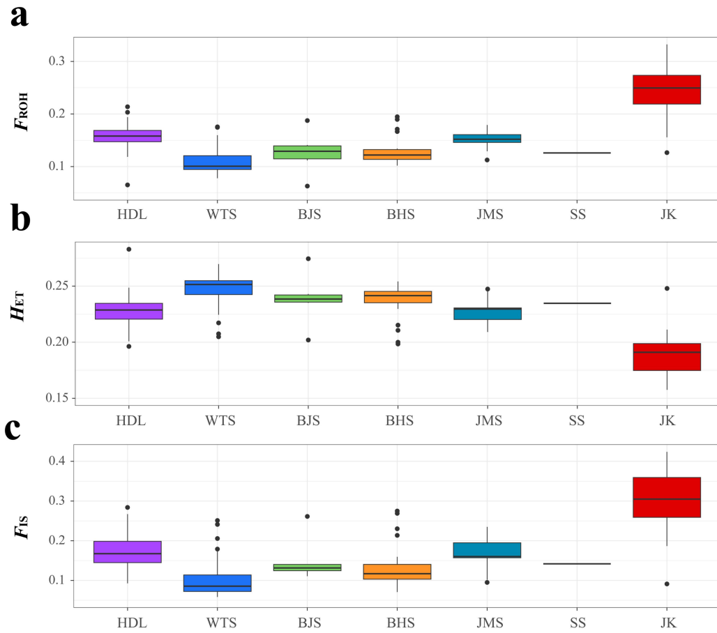
Figure S18. The fraction of the genome in Lonicera oblata populations. (a) the fraction of the genome in runs of homozygosity ( F_{ROH} ). (b) genomic heterozygosity ( H_{ET} ). (c) inbreeding coefficient ( F_{IS} ).
