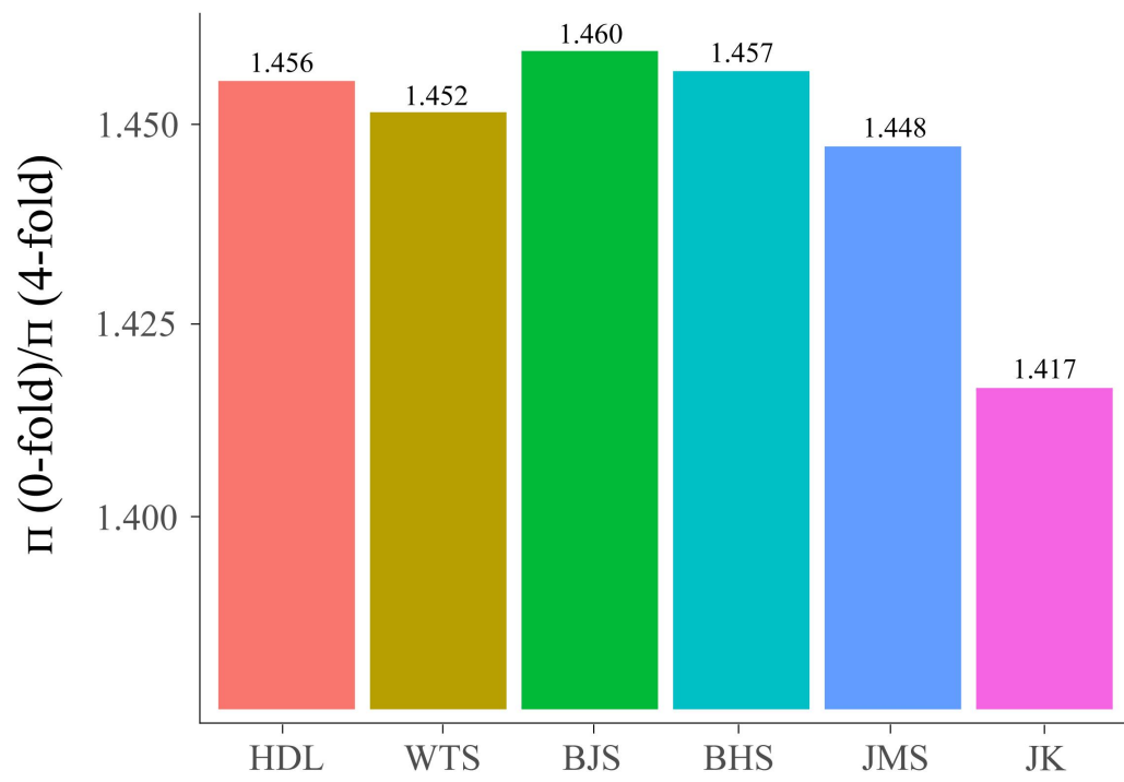
Figure S19. A comparison of \pi_0 / \pi_4 ratios in Lonicera oblata populations.
