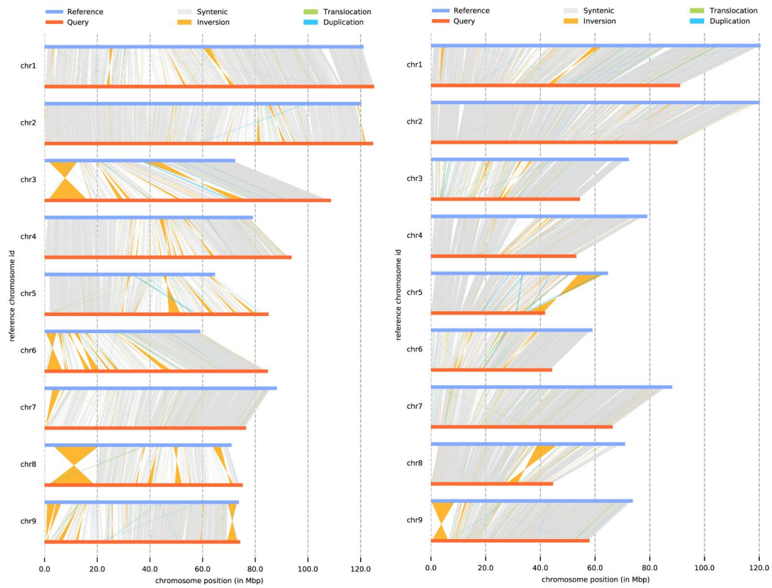
Figure S3. Comparative chromosome structure analysis in Lonicera . Left panel: L. oblata vs. L. japonica ; Right panel: L. oblata vs. L. maackii . The reference chromosome (in blue) is derived from L. oblata .
