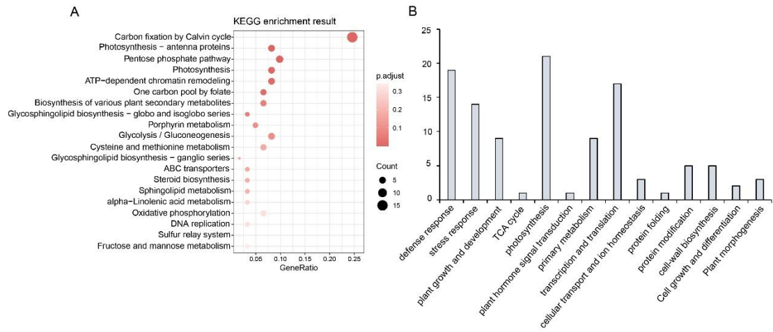
Figure S6. Functional analysis of proteins interacting with PfMLP25. (A). KEGG pathway enrichment analysis of PfMLP25-interacting proteins. (B). The histogram chart illustrates the distribution of PfMLP25-interacting proteins identified via GST pull-down MS screening, categorized based on function analysis.
