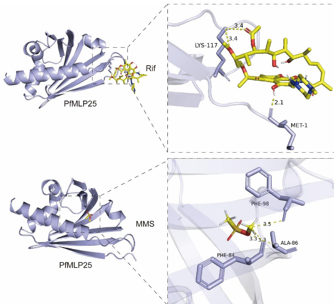
Figure S7. Molecular docking of PfMLP25 and two phytoplasma inhibitors. The molecular docking results of Rif and MMS with PfMLP25.
