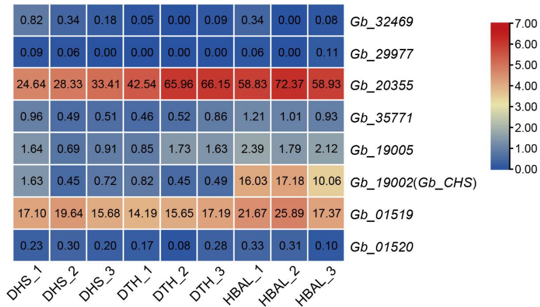
Fig. S9 Expression profiles of all eight CHS genes in three G. biloba cultivars with contrasting flavonoid contents.
