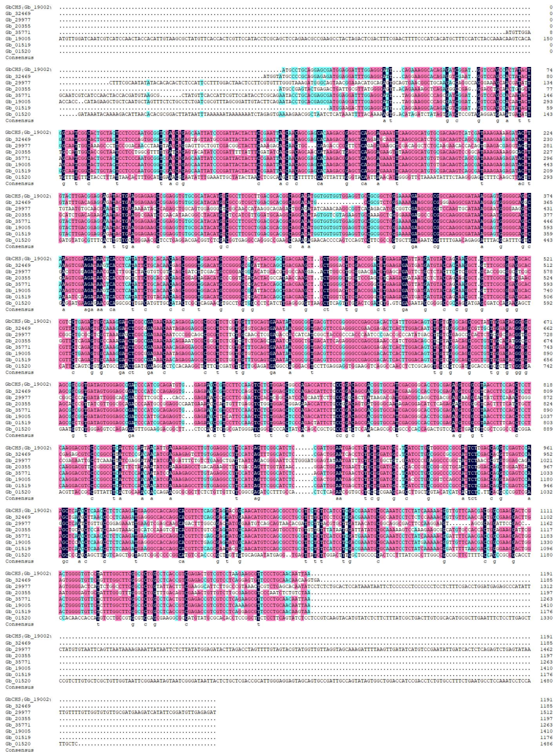
Fig. S8 Multiple sequence alignment of GbCHS ( Gb_19002 ) protein with other CHS family members in G. biloba .
