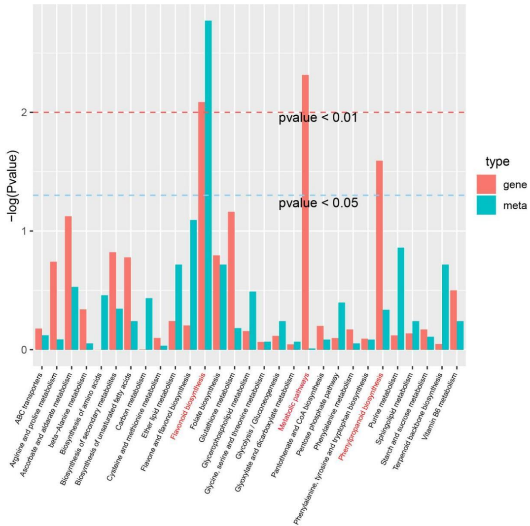
Fig. S5 KEGG enrichment analysis of DAMs and DEGs in 'DTH' vs. 'DHS' comparison.
