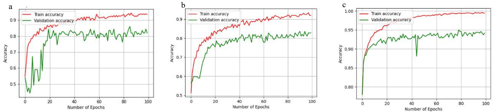
Supplementary Fig. S4. Training and validation accuracy curves of the convolutional neural networks shown in the step 1 of the Hybrid architecture. Figure (a), (b), and (c) represents the accuracies of the Arabidopsis thaliana , poplar ( Populus trichocarpa ) and maize ( Zea mays ) training data.
