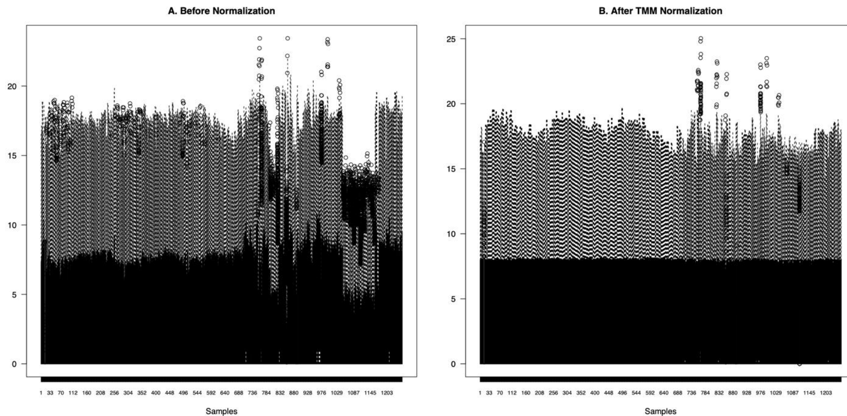
Supplemental Fig. S1. Box plots showing the distribution of read counts for Arabidopsis thaliana samples before and after TMM normalization. The x-axis represents individual samples, and the y-axis shows log-transformed read counts.
