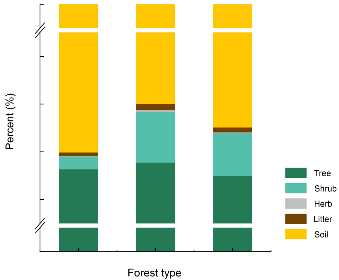
Fig. S1 Percentage contribution of different carbon pools to the total ecosystem carbon of the stand types.
