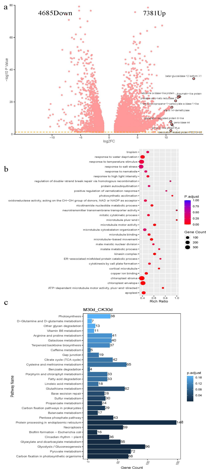
Supplemental Fig. S5 Transcriptome analysis. (a) Differentially expressed genes (DEG) between M30 d and CK30 d samples. (b) GO enrichment of DEG between M30 d and CK30 d. (c) KEGG enrichment of DEG between M30 d and CK30 d.
