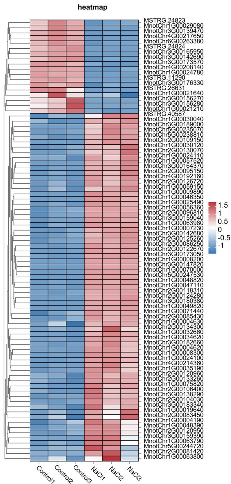
Figure S2. Heatmap analysis of differentially expressed plant hormone signal transduction pathway genes.
