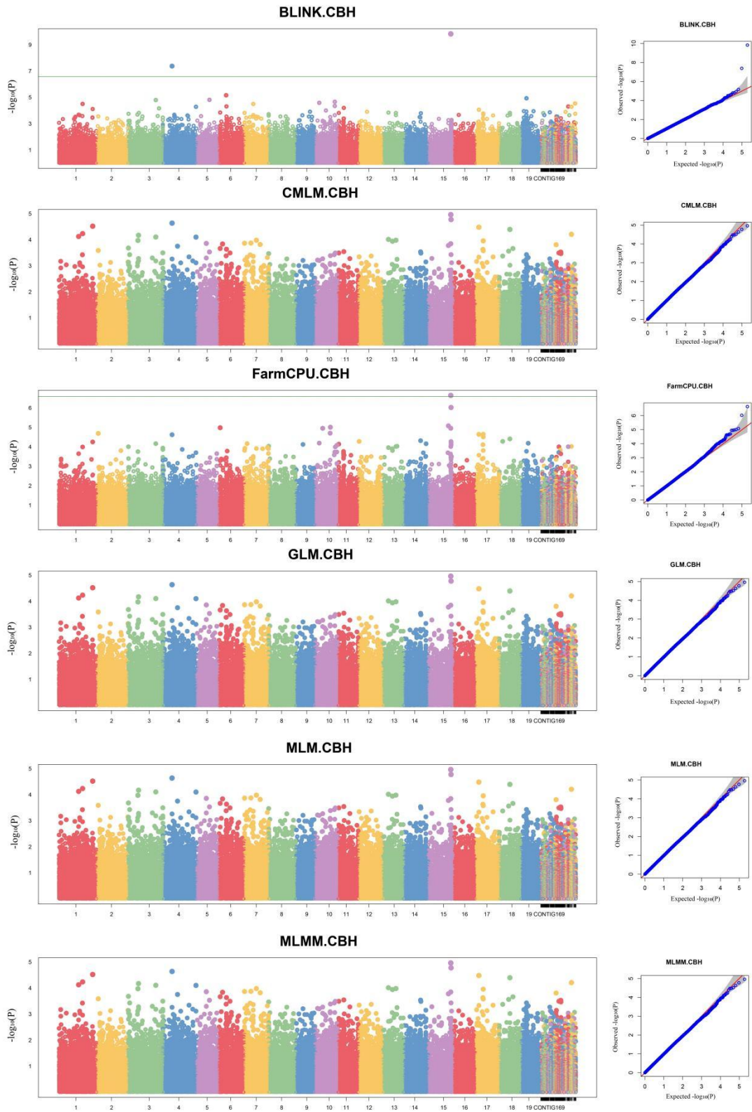
Fig. S11 Figure of the GWAS results for CBH using SNPs.
