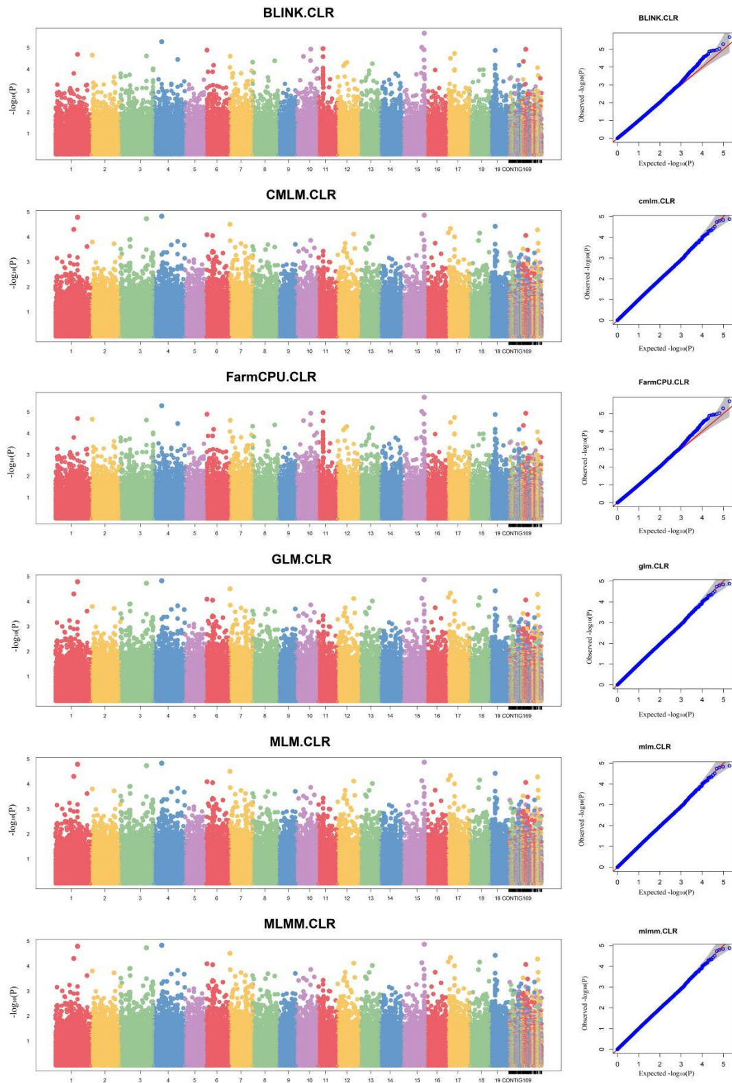
Fig. S7 Figure of the GWAS results for CLR using SNPs.
