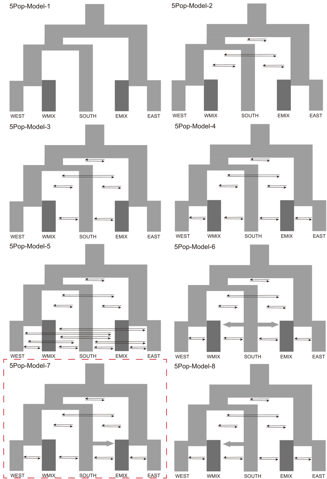
Figure S2 Diagram of 12 candidate demographic models of five clusters using fastsimcoal2.7.
