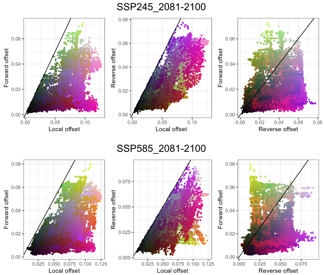
Figure S10 Bivariate scattergrams of local genetic offset, forward offset and reverse offset for SSP 245 (upper panel) and SSP 585 (lower panel) for 2081-2100. The color was identical to Fig. 6a.
