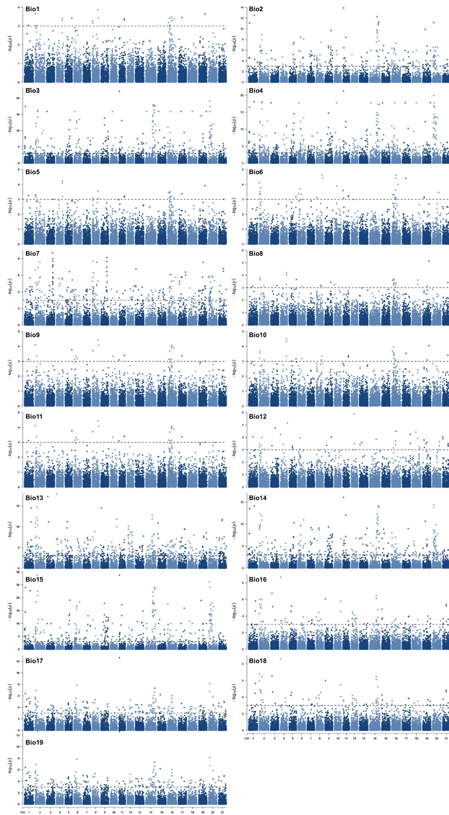
Figure S6 Manhattan plot of 16569 SNPs with 19 climatic variables in LFMM analysis.
