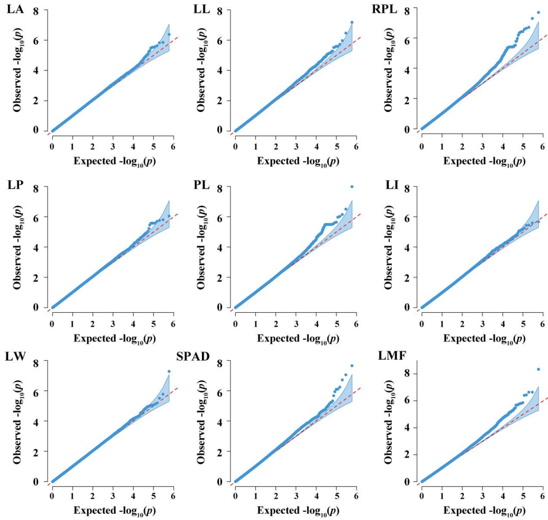
Supplementary Figure S3 QQ plot for single-trait GWAS analysis, corresponding to the manhattan plots for single-trait GWAS.
