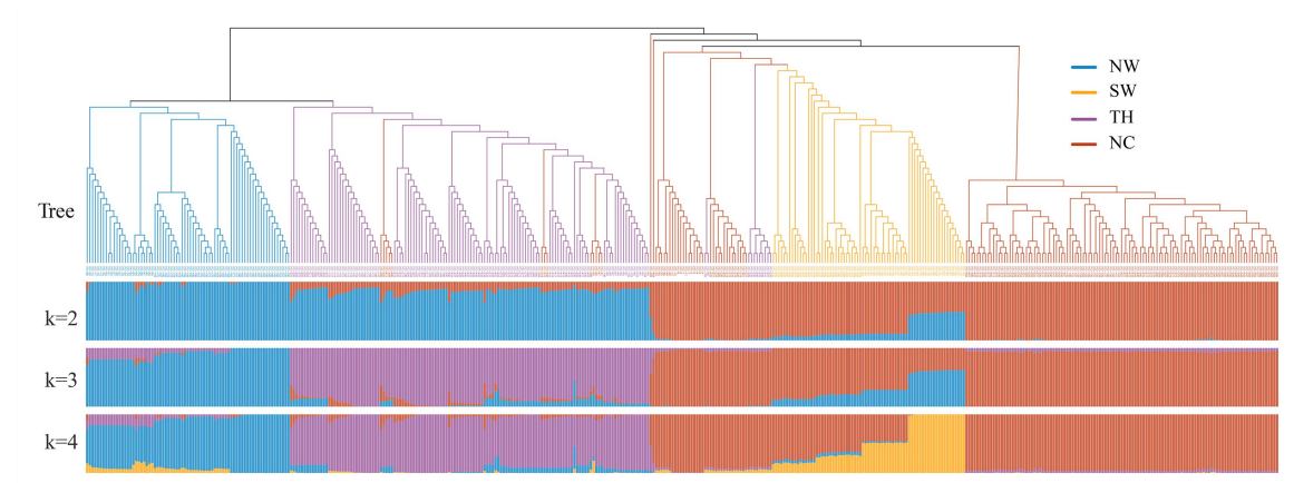
Supplementary Figure S1 Phylogenetic tree and population structure of P. cathayana populations [34] . Each individual is denoted by a vertical bar composed of different colors corresponding to its proportion of genetic ancestry.
