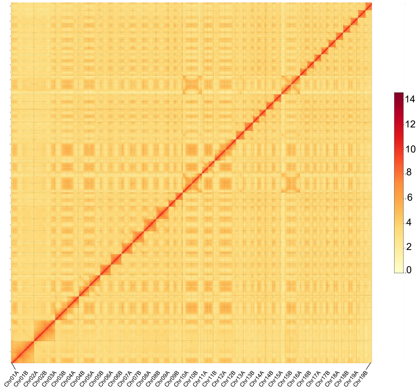
Fig. S2. Hi-C interaction matrix heatmap of NL895 diploid genome
