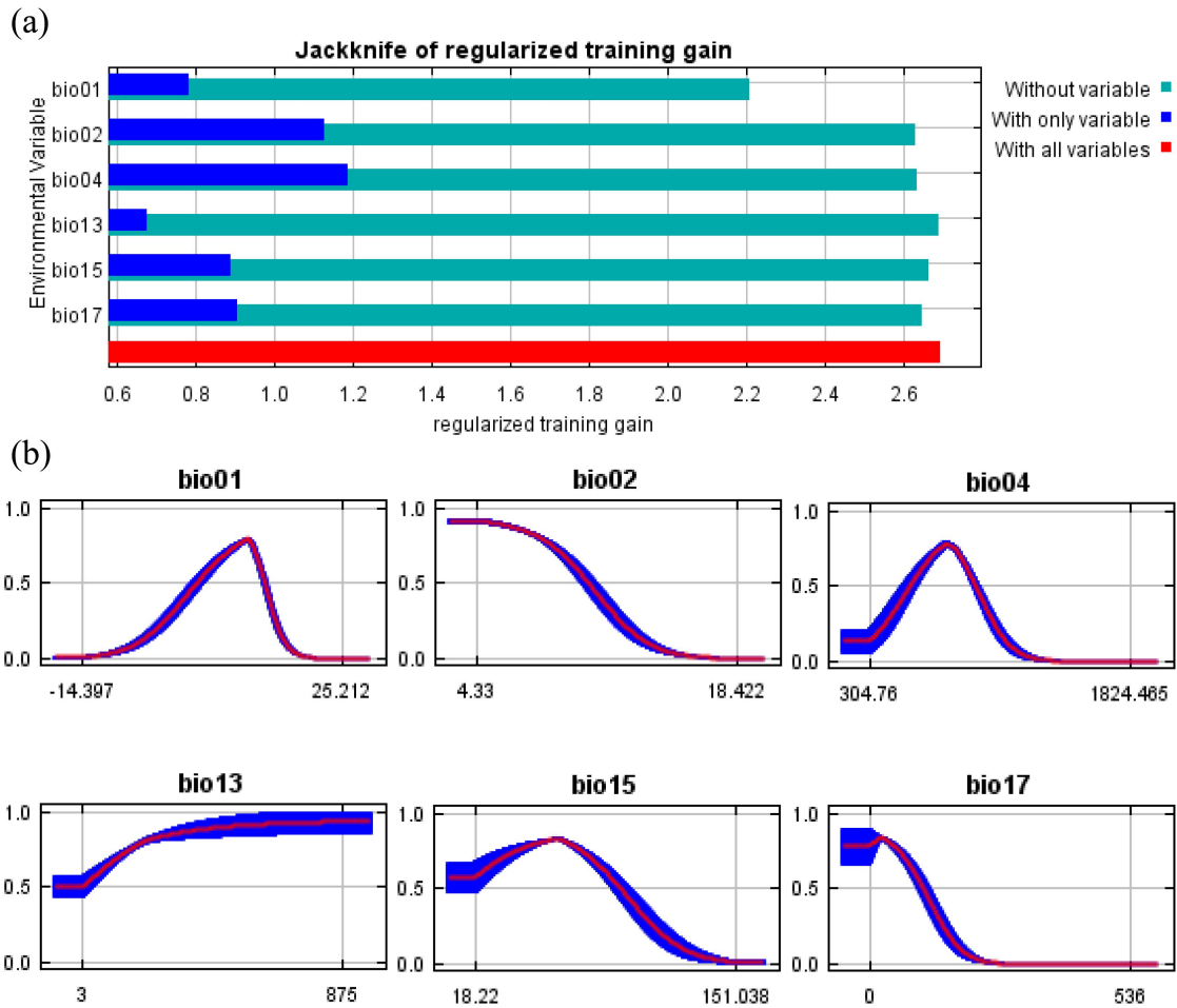
Fig. S9 (a) MaxEnt Jackknife tests of the environmental variables importance of Pterocarya hupehensis ecological niche model. (b) Marginal response curves of the predicted probability of occurrence for explanatory variables that contributed substantially to the MaxEnt model.
