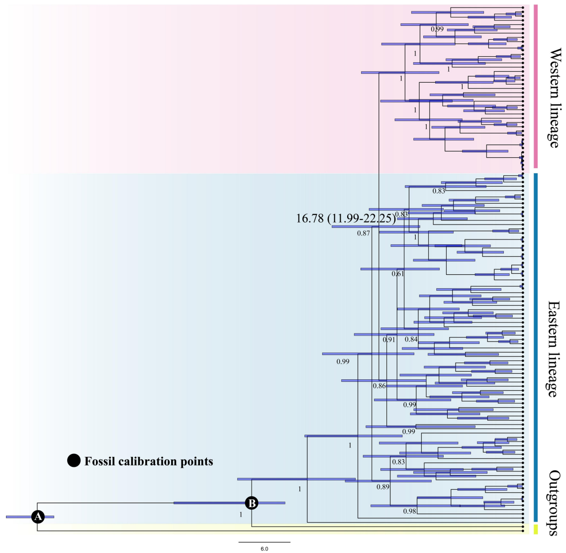
Fig. S6 The divergence time of the two major lineages of Pterocarya hupehensis inferred by BEAST based on the RAD-seq dataset. Blue bars indicate the 95% highest posterior densities (HPDs) of the time estimates.
