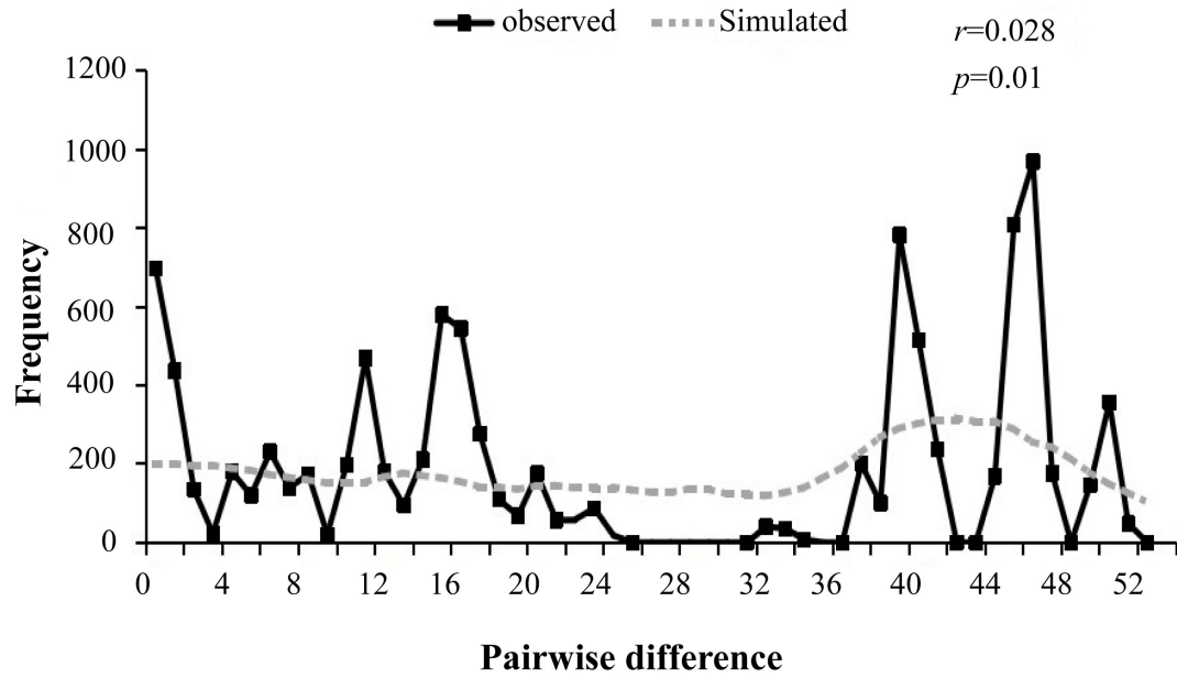
Fig. S2 Mismatch distribution for populations of Pterocarya hupehensis . The black and gray lines represent the observed and expected mismatch distributions, r represents the raggedness index, and p represents the significance of a simulation value greater than the observed value.
