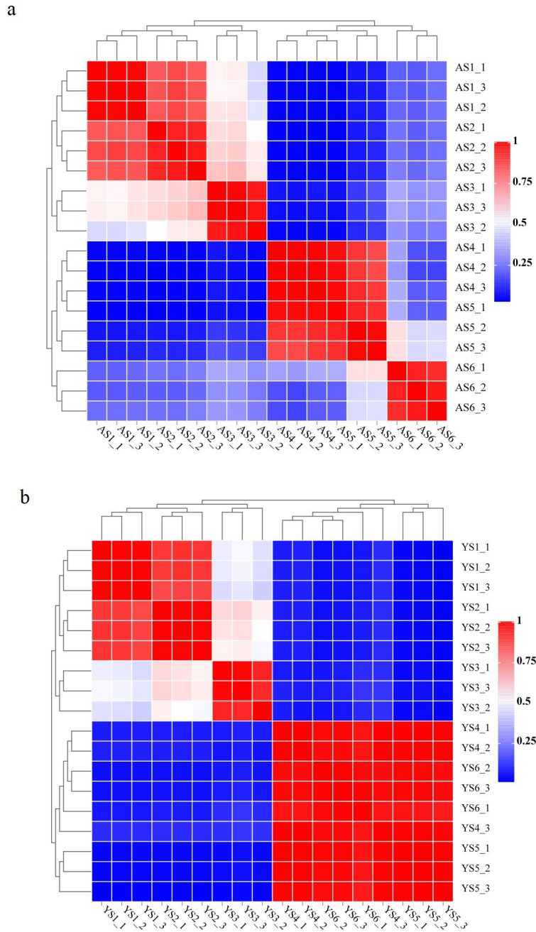
Supplemental Figure S1. Pearson correlation coefficient (PCC) analysis of gene expression data from the three replicate samples from each stage in bitter kernels (“Aohanqi-39” (AO, AS1~AS6)) and sweet kernels (“Youyi” (YY, YS1~YS6)). a. Pearson correlation coefficient (PCC) among the three biological replicates of six developmental stages in AO (AS1-AS6). b. PCC among the three biological replicates of six developmental stages in YY (YS1-YS6).
