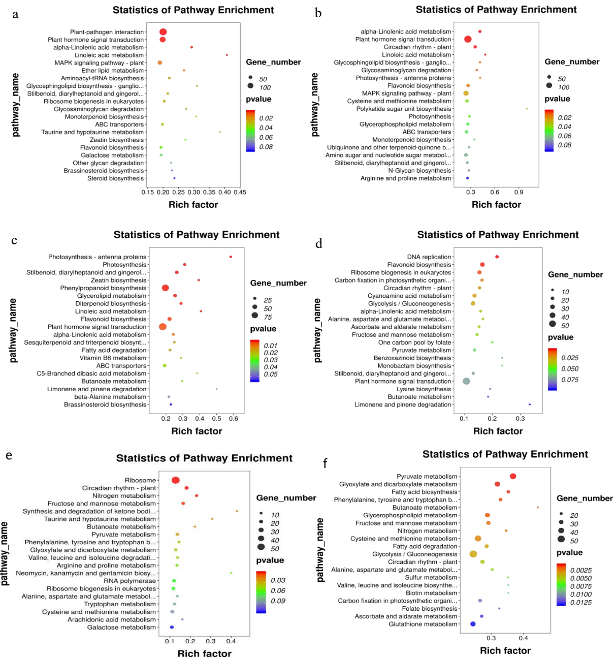
Supplemental Figure S4. KEGG pathway enrichment analysis of DEGs in the six different developmental stages comparison groups of “Youyi” (YY) and “Aohanqi-39” (AO). a~f were presented the KEGG enrichment of DEGs in stage of YS1 vs AS1 ~ YS6 vs AS6, respectively.
