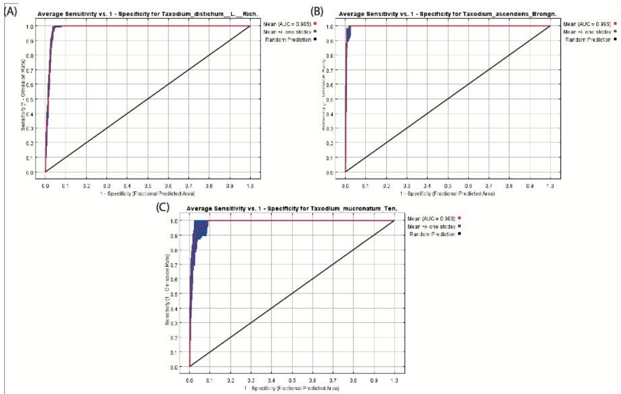
Figure S7. ROC plots for the three species models, with AUC values labelled top right. (A) T. distichum ; (B) T. ascendens ; (C) T. mucronatum ,
