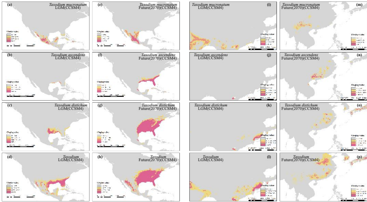
Figure S6. Species Distribution Modeling of the Three Taxodium Species in LGM and future 2070
