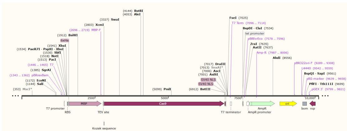
Figure S4. Representation of the full-length plasmid PMJ915. Streptococcus pyogenes Cas9 with two C-terminal SV40 NLS for nuclear localization; MBP, maltose binding protein labels; AmpR, ampicillin resistance; Multiple cloning sites for efficient gene insertion.
