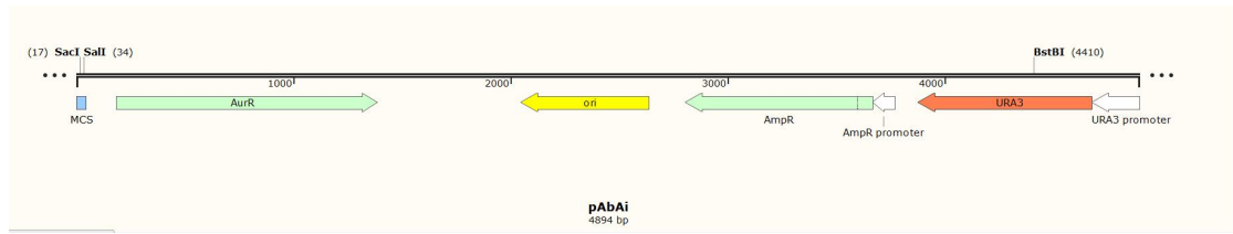
Figure S3. Schematic illustration of the full-length plasmid pAbAi. MCS, multiple cloning site; AurR, aureobasidin A-resistant; AmpR, ampicillin resistance; Sac I =unique Sac I restriction site within the plasmid; Sal I =unique Sal I restriction site within the plasmid; BstB I =unique BstB I restriction site within the plasmid
