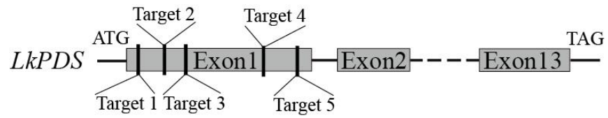
Figure S2. The predicted structure of LkPDS genes in the genome region. And the distribution position of the five targets in exon 1. The gray boxes indicate exons; the black lines represent introns.
