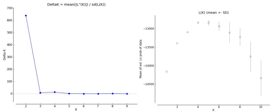
Figure S4. Estimated probability of the likelihood function according to Evanno's (2005) method for STRUCTURE analyses on 40 populations samples. The maximum \Delta K values correspond to the inferred true number of K clusters.
