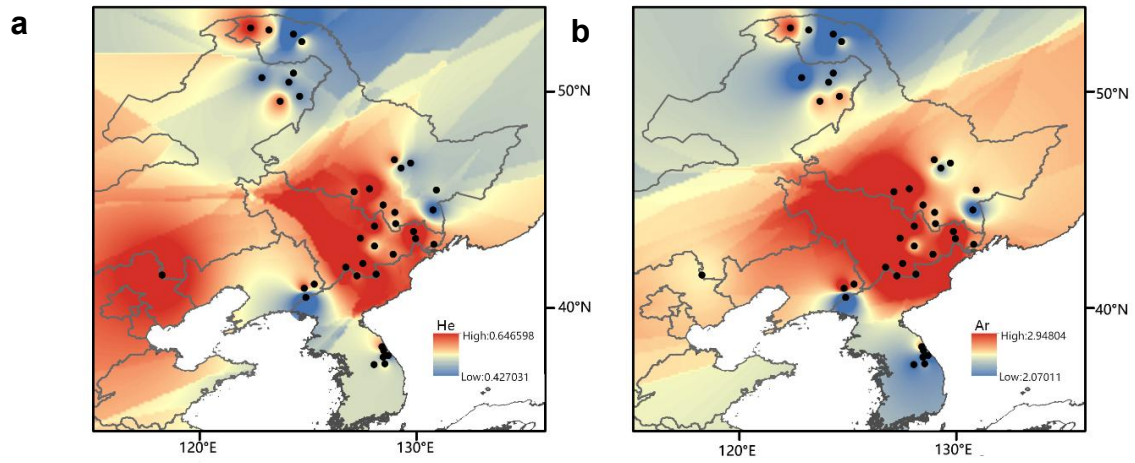
Figure S1. Spatial interpolation of expected heterozygosity ( H_e , a ) and allelic richness ( A_r , b ) among populations of Populus Koreana using inverse distance weighting (IDW) tool. Black dots denote sampling localities.
