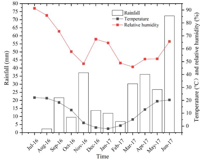
Fig. S1 Monthly variation in rainfall, temperature and relative humidity during the decomposition.
