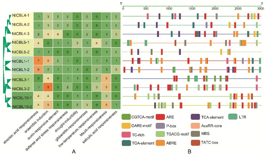
Figure S1 Cis -regulatory elements analysis of NtCBLs. (A) A heat map showing the number of cis -acting elements related to stress response in NtCBLs. (B) The distribution of cis -acting elements in the promoter region (ATG upstream) of NtCBLs, where different boxes represent different cis -acting elements.
