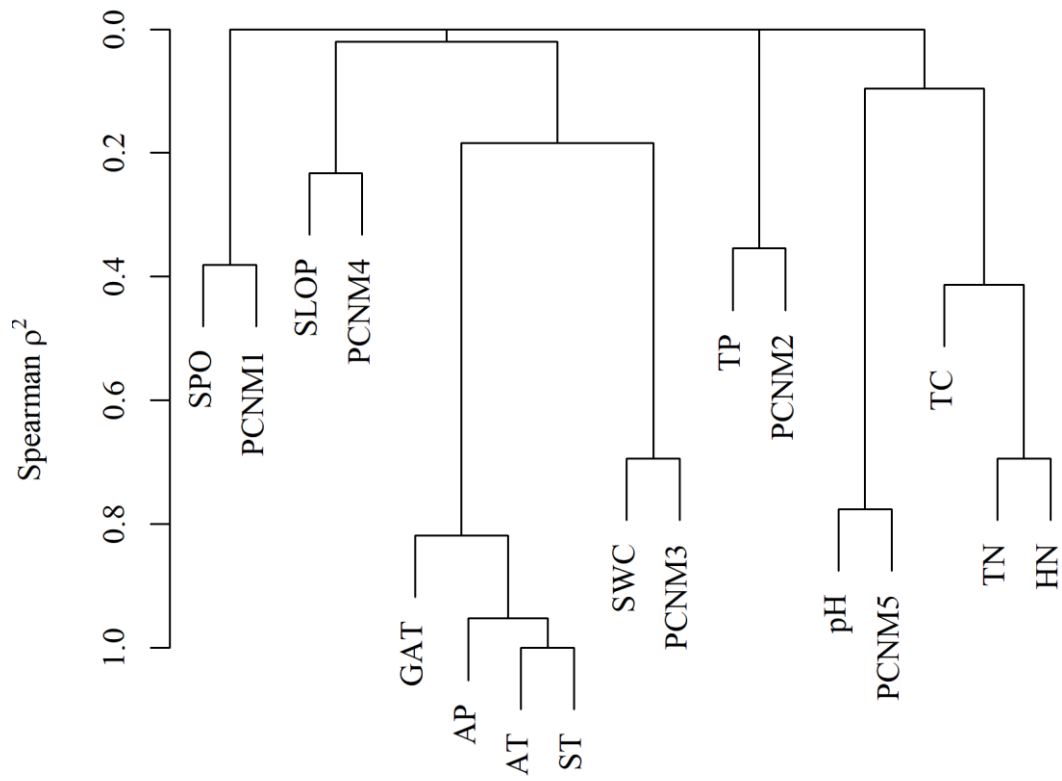
Supplemental Fig.S1 Multiple collinearity analysis of environmental variables. If Spearman \rho^2 > 0.5 , it can be inferred that there is a strong collinearity between these factors, and one of them kept while the others removed. We retained SPO, PCNM1, SLOP, PCNM4, AT, SWC, TP, PCNM2, pH and TC.
