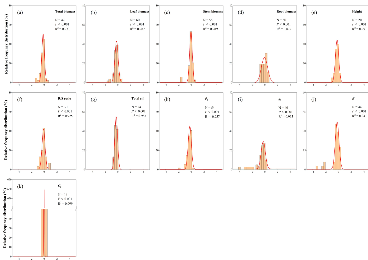
Figure S2 Frequency distribution of the data for heavy metal concentrations of (a) Total biomass, (b) Leaf biomass, (c) Stem biomass, (d) Root biomass, (e) Height (f) R/S ratio, (g) Total chl, (h) P_n , (i) g_s , (j) E , and (k) C_i
