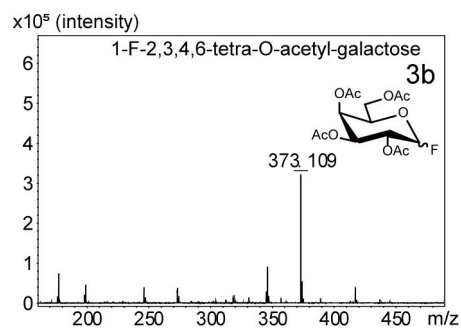
Supplementary Figure S2: Thin layer chromatography and MALDI-ToF-MS of 1-F-2,3,4,6-tetra-O-acetyl-glucose ( 3a ) and 1-F-2,3,4,6-tetra-O-acetyl-galactose ( 3b ). ii(a): fluorination of 1,2,3,4,6-penta-O-acetyl-glucose, ii(b): fluorination of 1,2,3,4,6-penta-O-acetyl-galactose, 3a: 1-F-2,3,4,6-tetra-O-acetyl-glucose, 3b: 1-F-2,3,4,6-tetra-O-acetyl-galactose.
