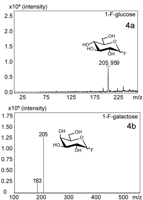
Supplementary Figure S3: Thin layer chromatography and MS analysis of 1-F-glucose ( 4a ) and 1-F-galactose ( 4b ). Glc=glucose standard, iii(a): deprotected 1-F-2,3,4,6-tetra-acetyl-glucose, Gal: galactose standard, iii(b): deprotected 1-F-2,3,4,6-tetra-acetyl-galactose; 4a :1-F-glucose, 4b :1-F-galactose.
