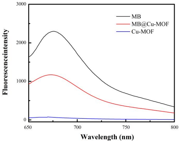
Figure S1. Fluorescence spectra of Cu-MOF, MB@Cu-MOF, and MB.
