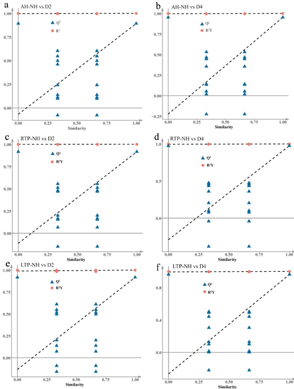
Fig. S5. 200 permutations test for the OPLS-DA model.
