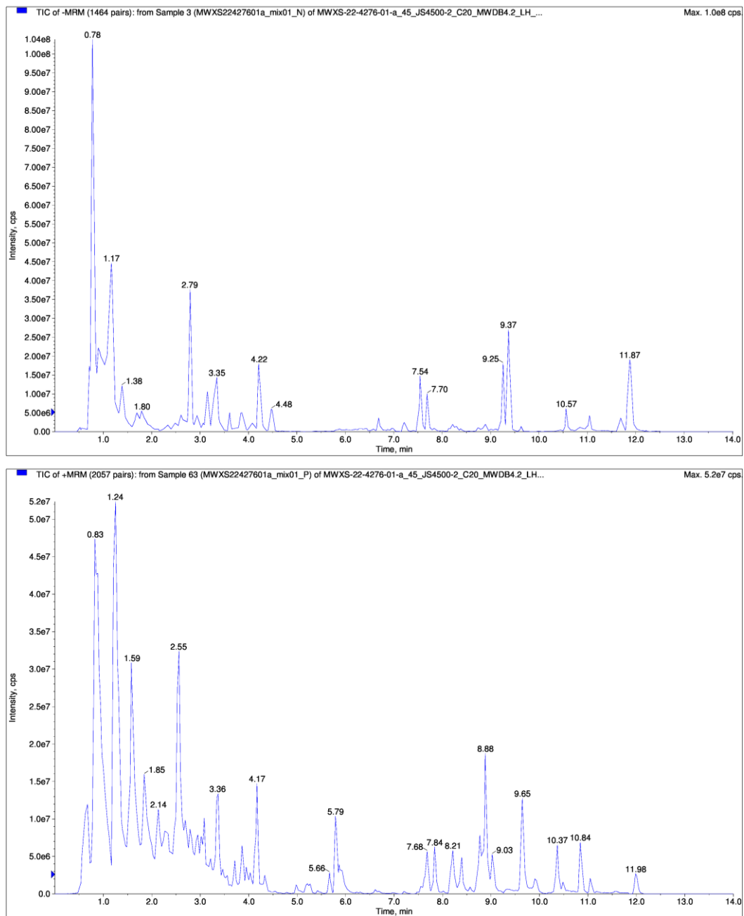
Fig. S4. Total ion flow map of mixed samples.
