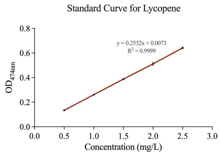
Figure S2 Standard curve for lycopene.
