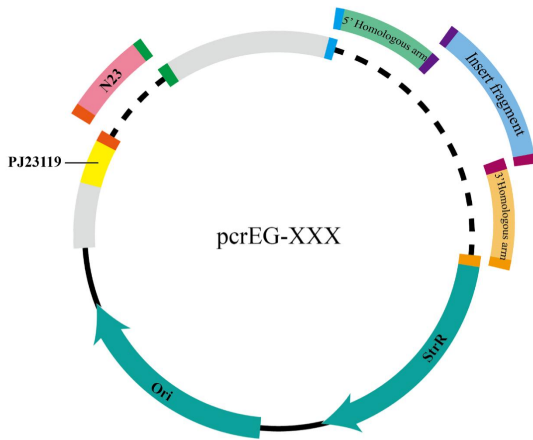
Figure S1 Schematic of pcrEG assembly. Dashed segments indicate regions that must be swapped between different pcrEG constructs; colored squares at the ends of each arc mark 15–20 bp homology arms used for fragment assembly.
