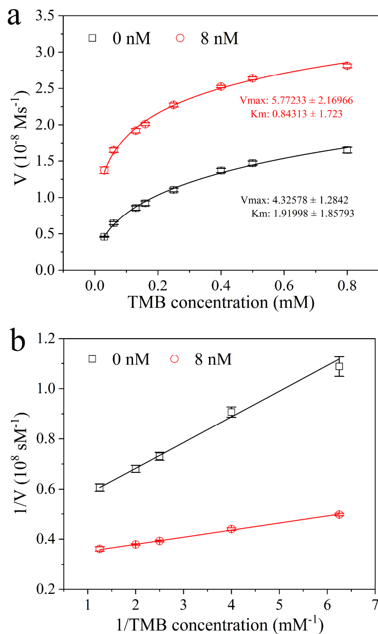
Figure S5 Steady-state kinetic analysis and the enzymatic mechanism of octahedral \text{Ag}_2\text{O} NPs catalyzed by P12-55 aptamer. (a) Michaelis-Menten plot. (b) Lineweaver-Burk plot.
