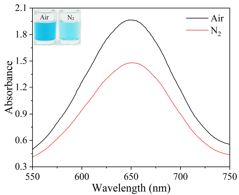
Figure S2 Comparison of TMB colorimetric reactions catalyzed by Ag 2 O NPs in air or N 2 -saturated buffer solutions.
