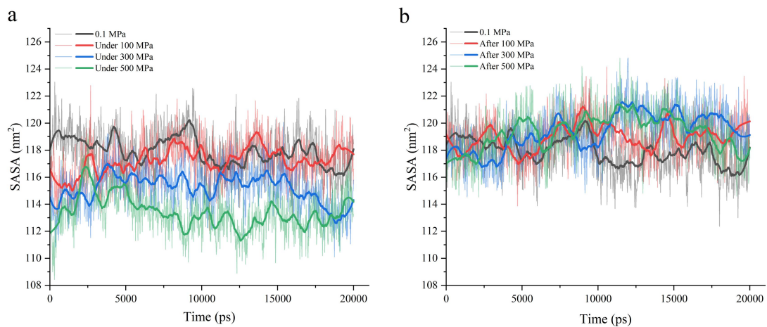
Fig. S3 SASA of PPO systems during the pressurization and depressurization stages from MD simulations. SASA plots of 0.1 MPa, under 100 MPa, under 300MPa, and under 500MPa (a), 0.1 MPa, after 100 MPa, after 300 MPa, after 500 MPa (b)
