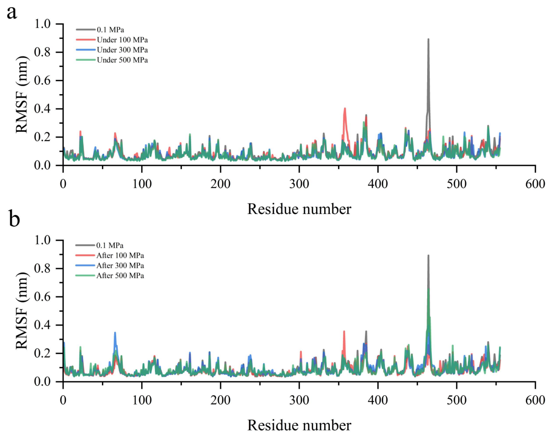
Fig. S2 RMSF of PPO systems during the pressurization and depressurization stages from MD simulations. RMSF plots of 0.1 MPa, under 100 MPa, under 300MPa, and under 500MPa (a); 0.1 MPa, after 100 MPa, after 300 MPa, after 500 MPa (b).
